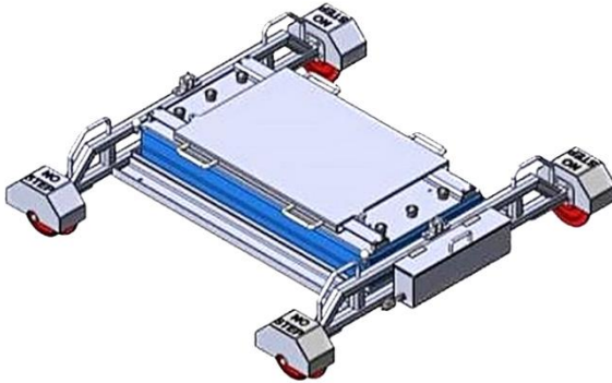
LIFT TABLE WITH BALL TRANSFER TABLE Item #0594-1
