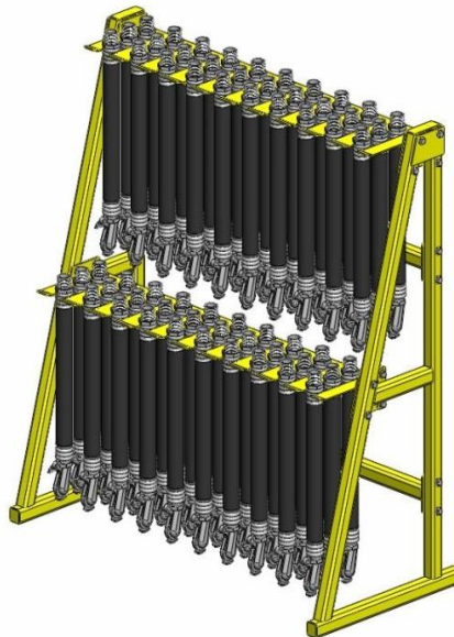
60 Unit Brake Hose Storage Rack
