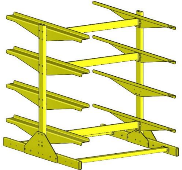
24 Unit Brake Beam Rack
