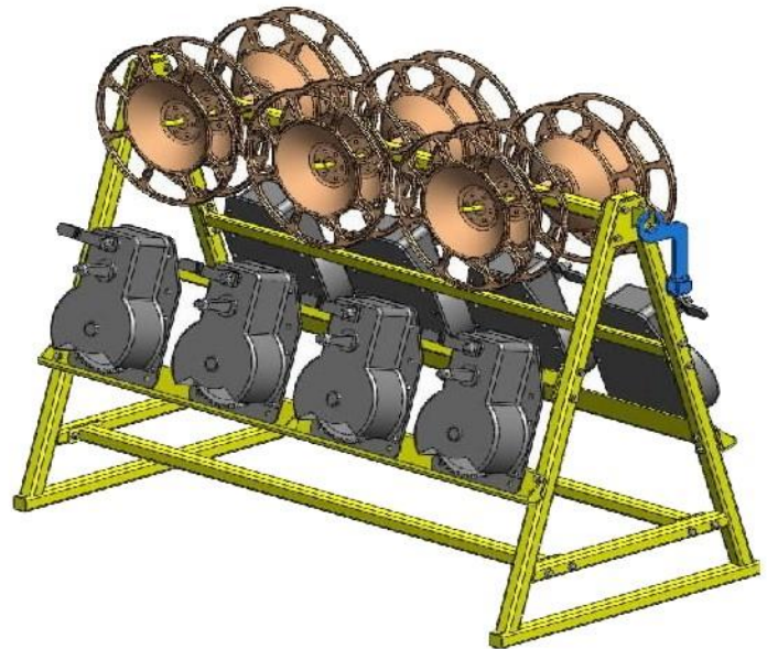
Double Sided Hand Brake Equipment Storage Rack W 77" X D 41" X H 59" Item # 0368
