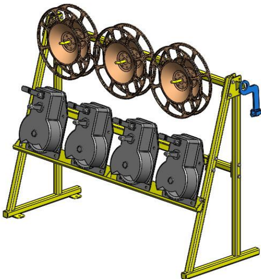
Single Sided Hand Brake Equipment Storage Rack W 77" X D 31" X H 59" Item # 0368-1
