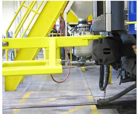
Stacking Fixture Item # 0032-4
