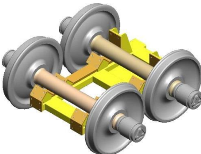
Double Wheel Set Caddy Item # 0288
