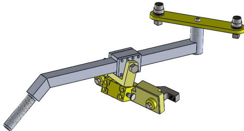
Tier 4 Hydraulic Torque Wrench Extension Arm for Connecting Rod (HYTORC AVANTI 1 Not Included) Item # 0499
