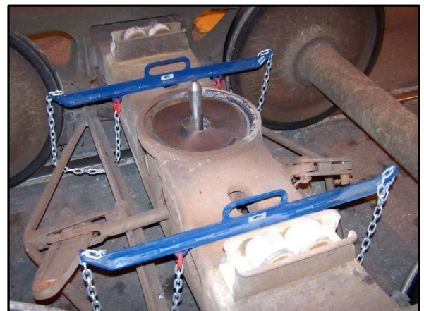
Brake Beam Support Fixture
