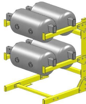
4 Unit Air Reservoir Rack
