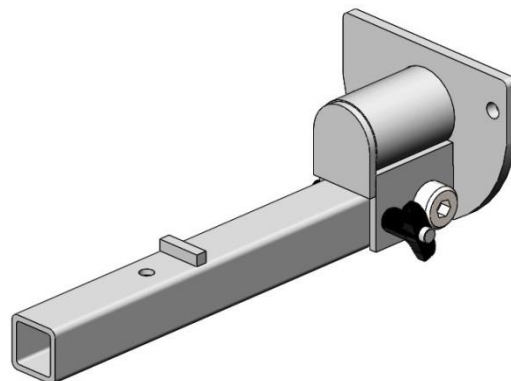
Graham White Electric Wheel Handbrake Lifter Used With Gieske C-Frame Item # 0525
