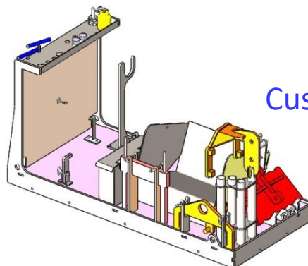
Transition Section Lifter Lifts GEVO Stage 1, Stage 2 & FDL Transition sections. Item # 0570
