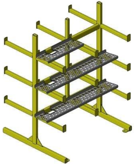
Cross Over Step Rack
