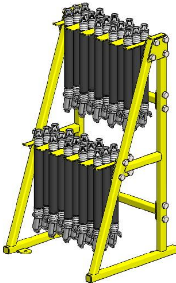
30 Unit Brake Hose Storage Rack
