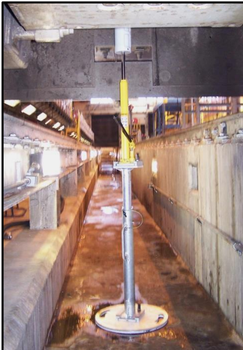
Adjustable Height Coupler Pin Lifter Item # 0310
