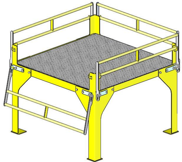
Knuckle Table 48" X 48" Item # 0033-15
