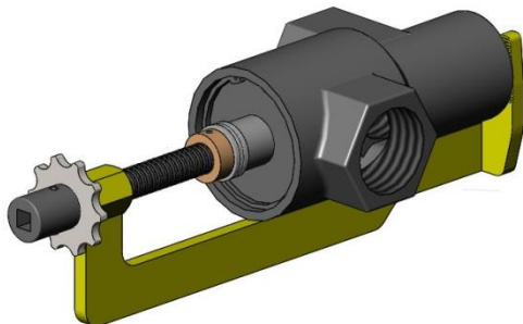
Locomotive ACE Starter Valve Compressor Item # 0556
