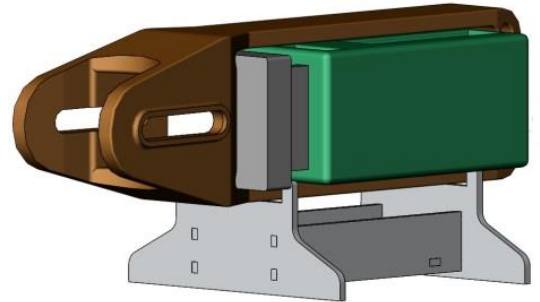
Aluminum Draft Gear Cradle Item # 0426
