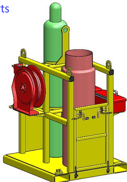
Forklift Torch Cart Item # 0377
