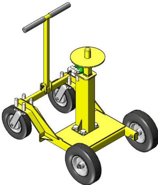
Center Plate Installation Cart
